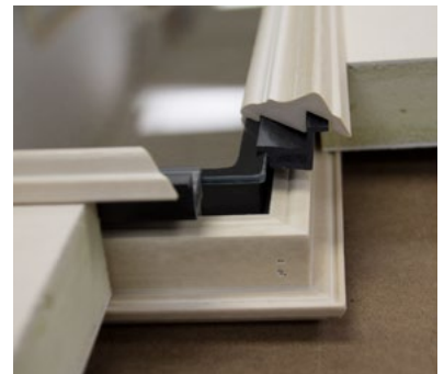
Patented frame design creates a strong and moisture-proof barrier.
